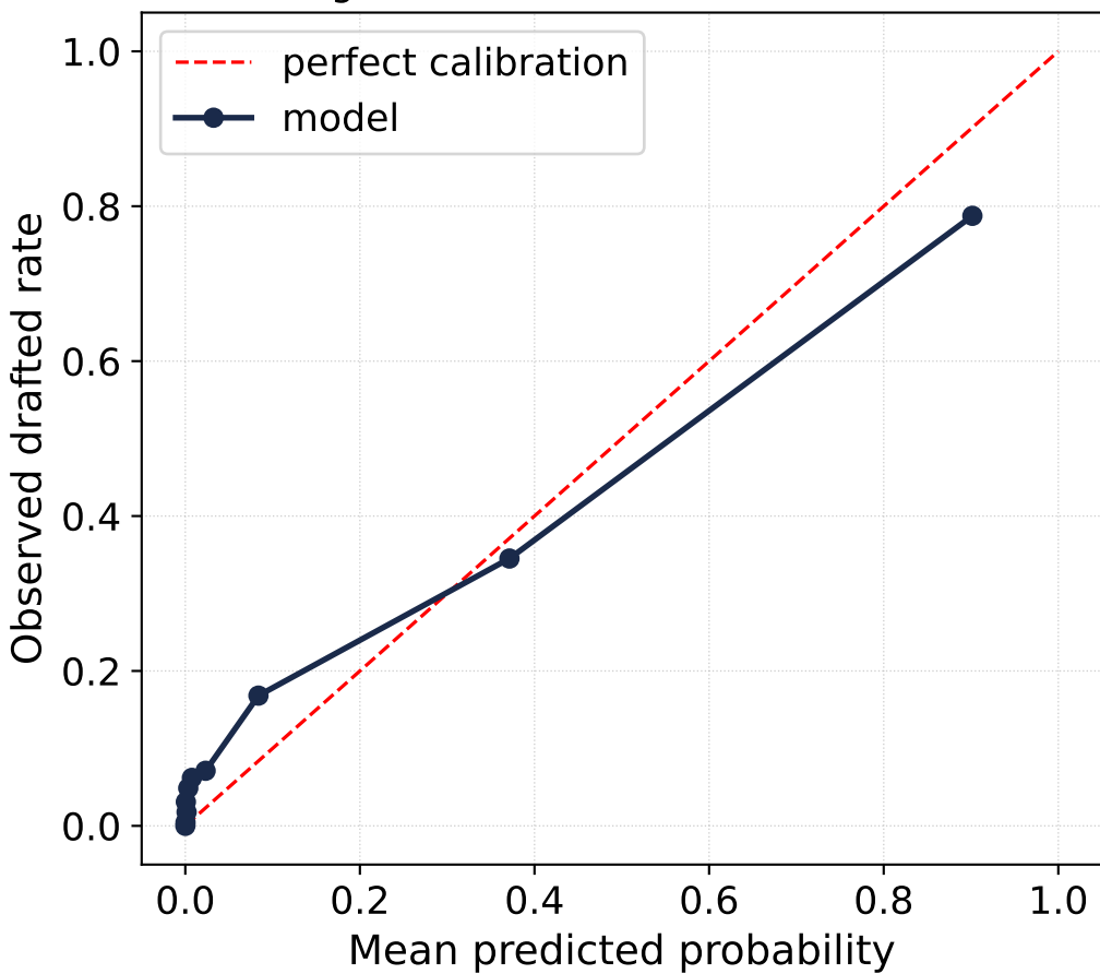
Stage 1 - Draft Classifier - Calibration
